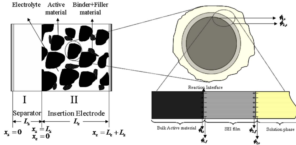
Figure 1. (Color online) Schematic of a foil/separator/porous insertion electrode cell sandwich. On the right: schematic of the magnified version of the interface showing the film at the electrode/electrolyte interface.
