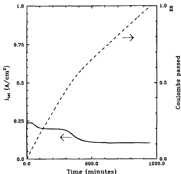
Fig. 12. Divided cell current density and coulombs passed vs. time when E_{\text{cell}} = 3.0 \text{ V} .
