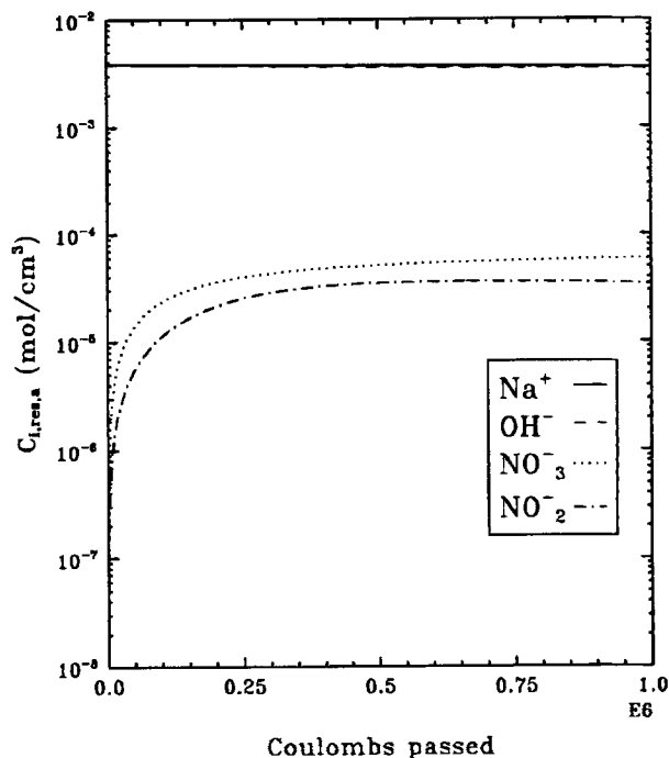
Fig. 6. Divided cell anolyte reservoir ionic concentrations vs. coulombs passed when E_{\text{cell}} = 3.5 V.
