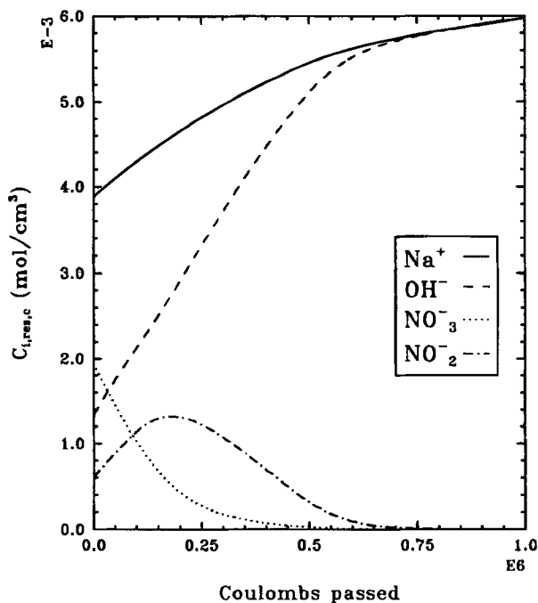
Fig. 10. Divided cell catholyte reservoir ionic concentrations vs. coulombs passed when E_{\text{cell}} = 3.0 \text{ V} .
