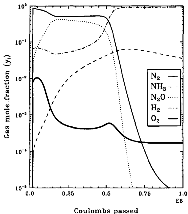
Fig. 11. Divided cell catholyte off-gas composition (mole fraction) vs. coulombs passed when E_{\text{cell}} = 3.0 \text{ V} .
