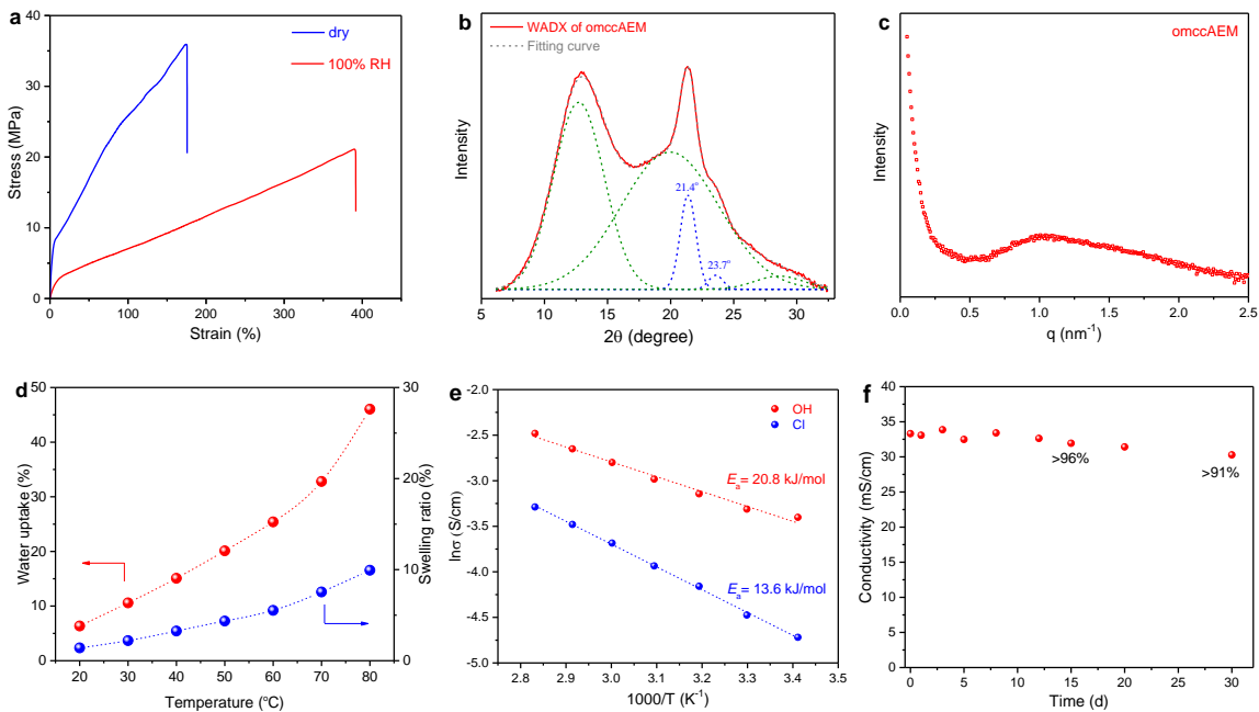
Figure 4.4. a. Stress-strain curves of omccAEM membrane in a dry state and a hydrated condition; b. WADX pattern of omccAEM membrane (red line: experimental data; grey line: fitting sum curve; green and blue lines: fitting multi-peaks, where blue line is considered as a crystalline peak); c. SAXS profile of omccAEM membrane; d. water uptake and swelling ratio for omccAEM membrane at different temperature; e. Arrhenius plots for conductivity of omccAEM with chloride and hydroxide as a function of temperature under fully hydrated conditions; f. room temperature conductivity as a function of immersion time of omccAEM in 3M KOH aqueous solution at 60 °C.
