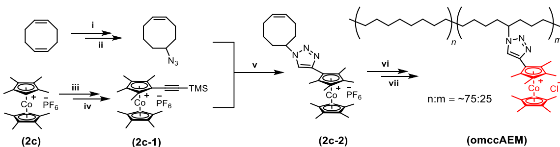
Figure 4.2. Synthesis of octamethyl cobaltocenium polyelectrolytes as AEMs. (synthesis details. i : HBr/HAc; ii : NaN 3 , DMF, 70 °C; iii : ethynyltrimethylsilane, n -BuLi, THF; iv : triphenylcarbenium hexafluorophosphate, DCM; v : CuSO 4 , Na ascorbate, THF/H 2 O; vi : Grubbs III catalyst, DMAc/xylenes, p -toluenesulfonyl hydrazide, Bu 3 N; vii : aqueous NH 4 Cl, ion-exchange resin, 60 °C)
