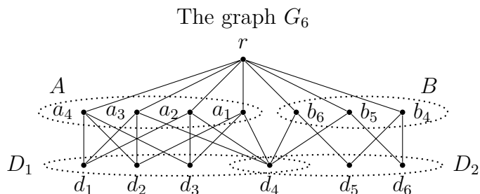
Figure 3.8 The graph G_6 . All vertices are shown.
