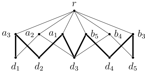
Figure 3.9 Steiner trees in the graph G_5 for D as in Definition 3.5 and the vertex set V_1 as above. The Steiner trees are in bold.
