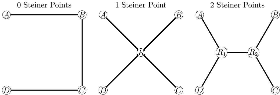
Figure 1.1 Spanning trees for the unit square using 0, 1, or 2 Steiner points. The Steiner points are labeled by the letter R .
