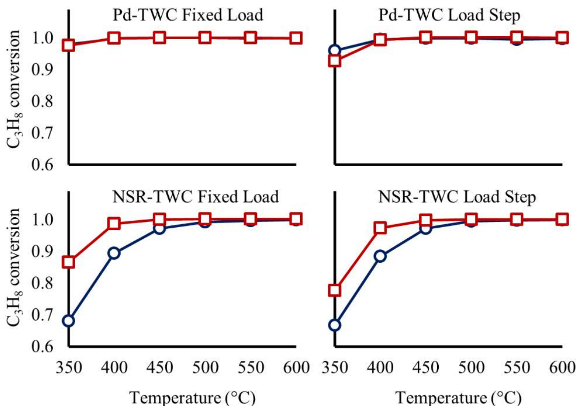
Figure 3.14: Average C_3H_8 conversion for Pd-TWC (top) and NS-TWC (bottom) for both fixed load (left) and load step (right) conditions comparing degreened (circles) and aged (squares) samples
