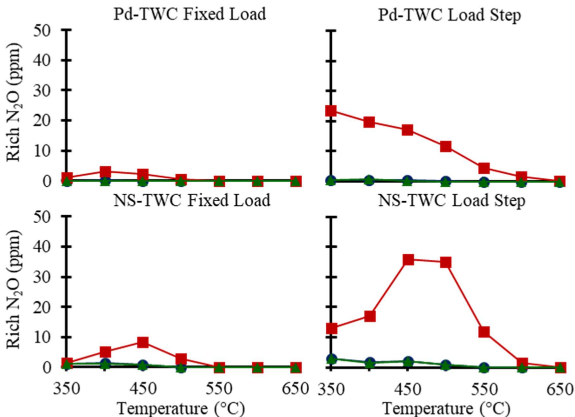
Figure 4.11: Clean (blue), Sulfated (red), and Desulfated (green) rich phase N_2O production for the Pd-TWC (top) and THE NS-TWC (bottom) under Fixed Load (left) and Load Step (right) conditions
