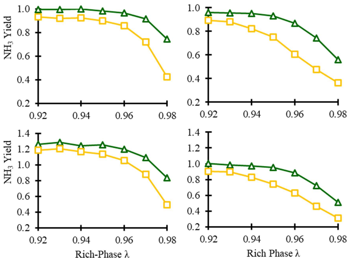
Figure 6.2: The production of NH 3 based on rich phase \lambda for Malibu-1 (top) and ORNL-1 (bottom) at 350°C (left) and 550°C (right) under fixed load conditions.
