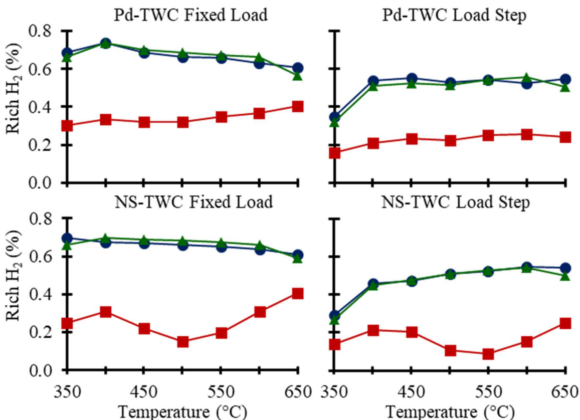
Figure 4.14: Clean (circle), Sulfated (square), and Desulfated (triangle) rich phase H_2 concentration for the Pd-TWC (top) and THE NS-TWC (bottom) under Fixed Load (left) and Load Step (right) conditions
