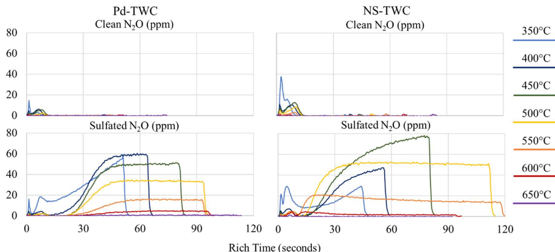
Figure 4.12: Isolated rich phases for \text{N}_2\text{O} production during fixed load operation over the Pd-TWC (left) and the NS-TWC (right) under clean (top) and sulfated (bottom) conditions.
