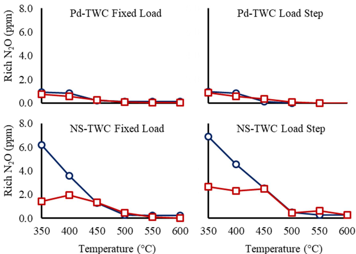
Figure 3.12: Average rich phase \text{N}_2\text{O} production for the Pd-TWC (top) and the NS-TWC (bottom) for both fixed load (left) and load step (right) conditions comparing degreened (circles) and aged (squares) samples
