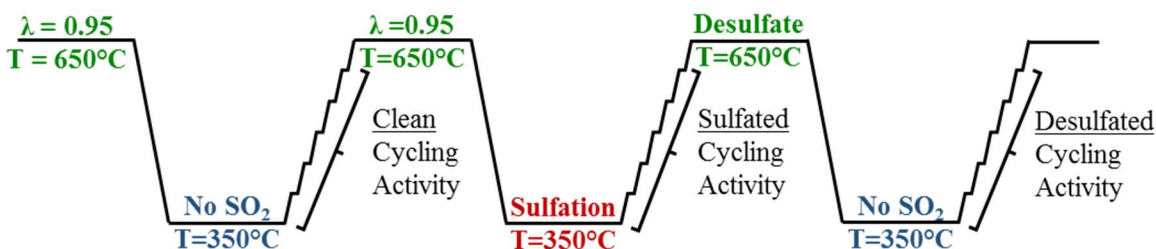
Figure 4.1: Procedure for long term sulfation experiments
