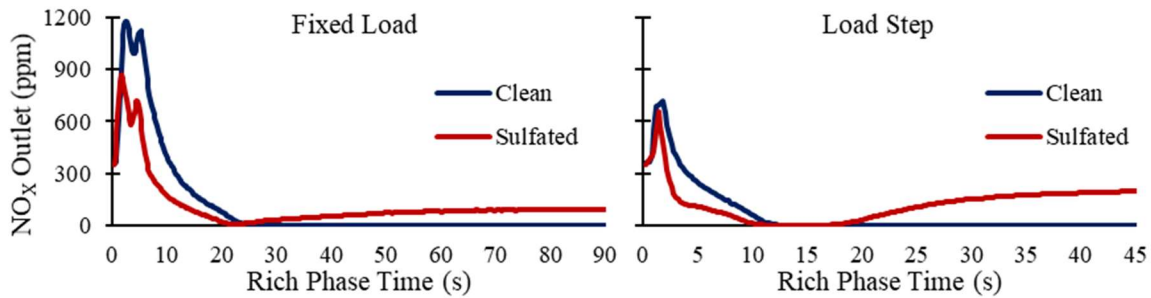
Figure 4.10: Rich phase breakthrough of \text{NO}_x on the NS-TWC catalyst before and after sulfation at 500^\circ\text{C} .
