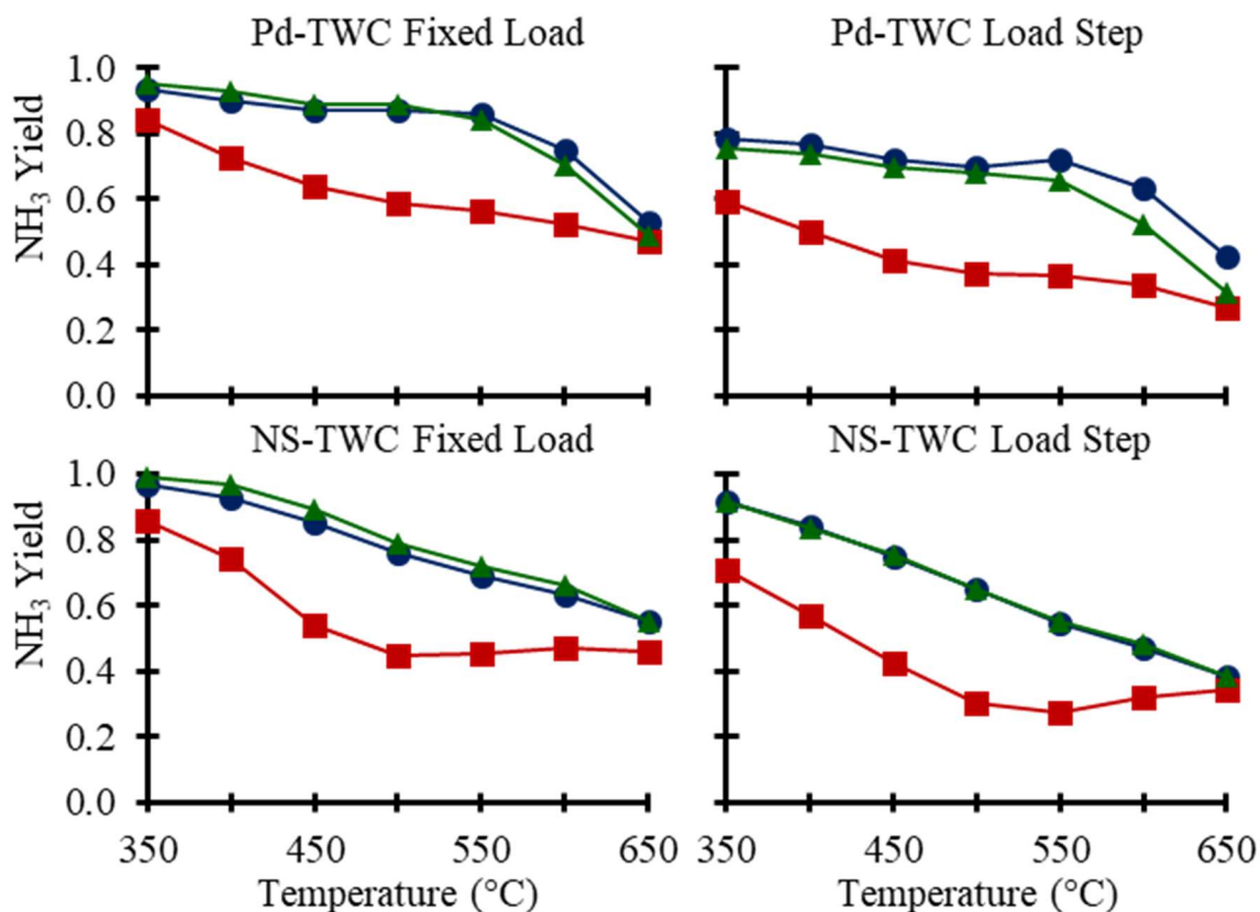
Figure 4.7: Clean (circles), sulfated (squares), and desulfated (triangles) \text{NH}_3 production for the Pd-TWC (top) and the NS-TWC (bottom) under Fixed Load (left) and Load Step (right) conditions
