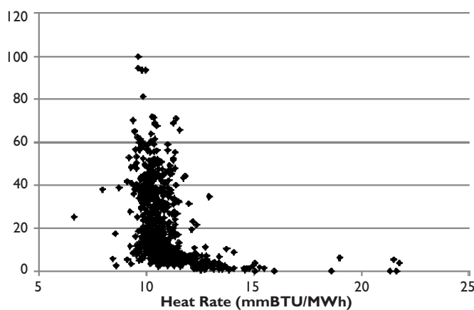
Figure 2. Distribution of Heat Rates Across U.S. Coal Fleet in 2008
