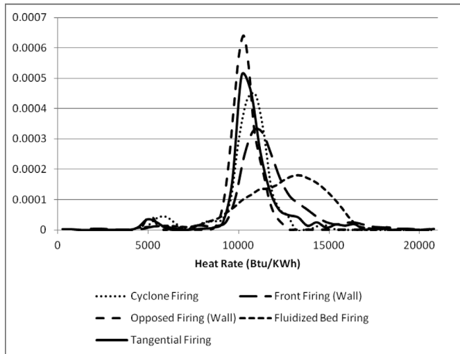
Figure 3. Distribution of Heat Rates by Boiler Technology
