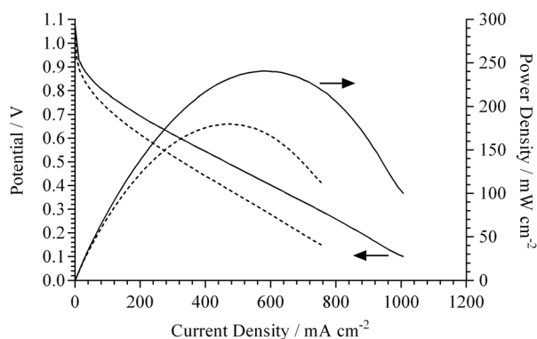
Fig. 6 Beginning of life fuel cell performance curves at 50^\circ\text{C} for MEAs containing electrodes fabricated using either 15% mass (dashed line) or 20% mass (solid line) RG powder AEI(OH - ). AAEM(OH - ) = ETFE RG type ( 80 \mu\text{m} fully hydrated thickness). H 2 /O 2 gases were supplied at 400 \text{ cm}^3 \text{ min}^{-1} and RH \approx 100\% . Data recorded from high current density to open circuit voltage at 10 \text{ mV s}^{-1} sweep rate.
