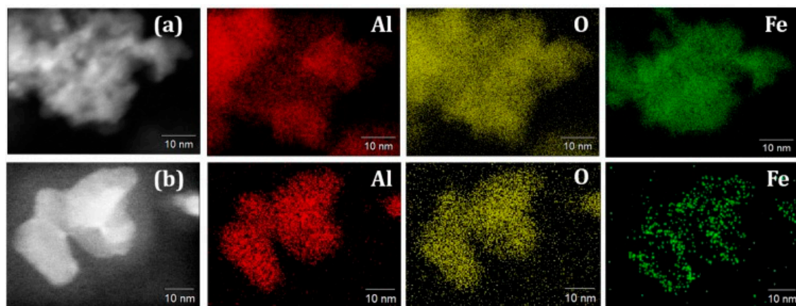
Figure 7. Representative HAADF-STEM images with corresponding EDS mapping of (a) \text{Fe}_2\text{O}_3 added onto a high-surface area \text{Al}_2\text{O}_3 support by metal salt impregnation and (b) \text{Fe}_2\text{O}_3 deposited onto the \text{Al}_2\text{O}_3 support by ALD [71]. EDS mapping of Al, O, and Fe shows rich Fe signals on the edges on the ALD-modified \text{Al}_2\text{O}_3 support, while there was no preferential distribution of Fe on the infiltrated sample. Reprinted with permission from Appl. Catal. A 2017 , 534, 70–77. Copyright (2017) Elsevier.
