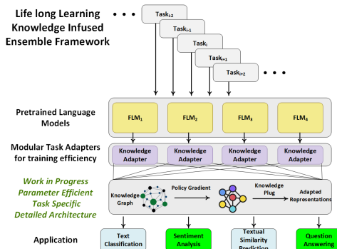
Figure 2: A framework for Lifelong Learning using Ensemble of FLMs. Blue tasks are the parts that have been implemented, and green parts are works in progress.
