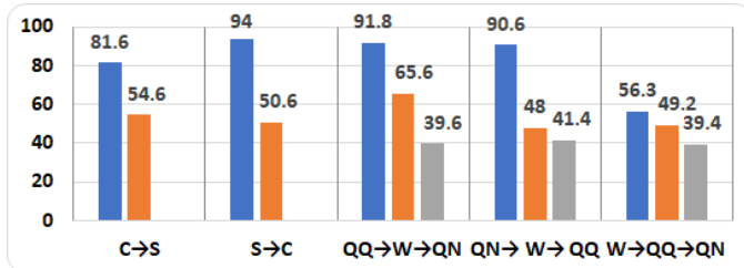
Figure 1: Performance (%) of the Fine-Tuned BERT_{base} on Continual Sequence of Similar GLUE Benchmark Tasks (C: CoLA, S: SST2, QQ: QQP, W: WNLI, QN: QNLI). Notation “C → S” denotes training on CoLA and testing on SST2. Notation “QQ → W → QN” indicates that the model underwent training on QQP, followed by WNLI, and was subsequently tested on QNLI.
