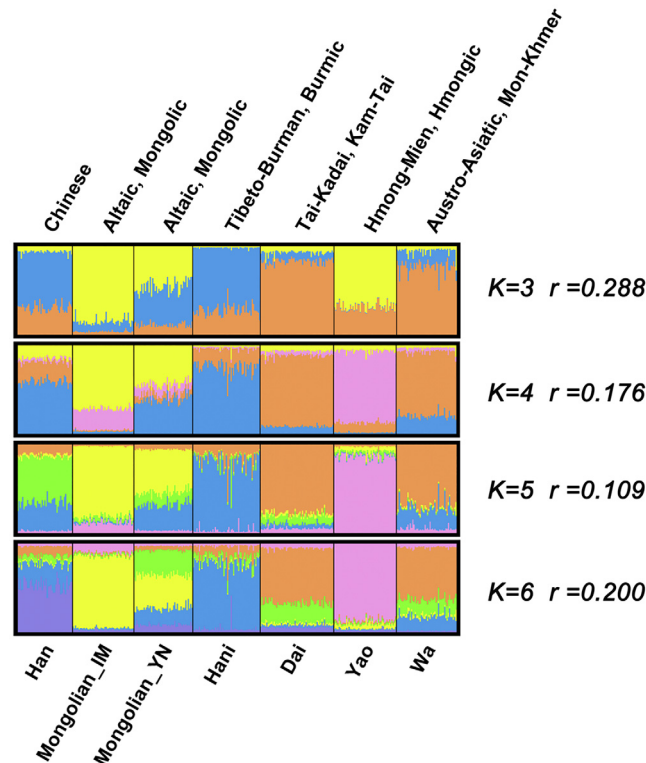
Fig 2. Clustering analysis from STRUCTURE. Population structure was investigated using STRUCTURE software, assuming K = 3, 4, 5, and 6 . Populations were ordered according to their linguistic affiliations. Linguistic affiliations and population names are labeled above and beneath the plot. According to the guidelines in the STRUCTURE manual and \Delta K values at different K s, K = 5 is the most appropriate value. The r values indicate that more information is given with the LOCPRIOR model than without it.
