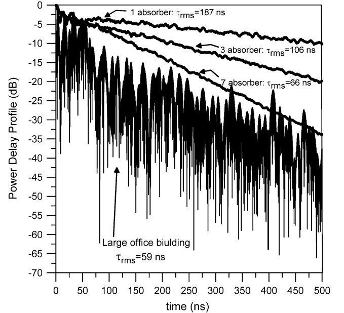
Fig. 2. Power delay profile from NIST measurements of the outdoor-to-indoor propagation channel in a 60-story office building. The lower curve is the instantaneous (thus, jagged) power delay profile measured in the building, and the three upper curves are power delay profiles generated by averaging 100 loaded reverberation chamber measurements [11].
