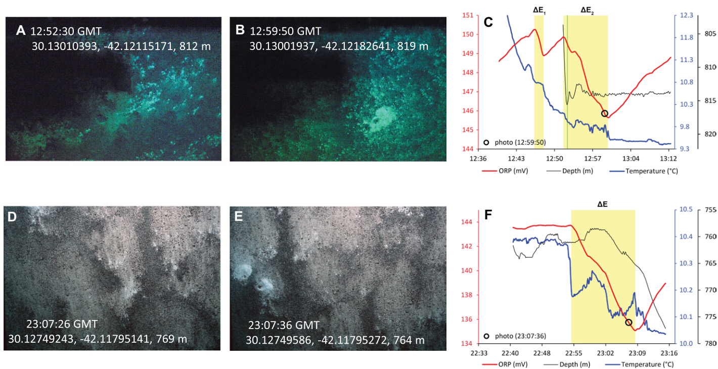
Figure 2. (A–F) Visual and sensor evidence of reduced fluids at the top of the Atlantis Massif collected during two remotely operated vehicle Jason transects. Images captured when vehicle was 4.2–4.5 m above the seabed depict typical sediments (A, D), in contrast to orifices surrounded by bright white sediments (B, E). Graphs show oxidation reduction potential (ORP) signal versus time in GMT (red line) and temperature versus time (blue line). Depth (black line) is shown when vehicle was <5 m above seafloor; changes are due to topography. (C) Graph depicts two substantial drops in ORP ( \Delta E ); drops >0.5 mV are diagnostic of reducing hydrothermal effluent (Text S1 [see footnote 1]). \Delta E_1 = -1.4 mV (from 12:46–12:48:16 h) corresponds to descent of vehicle through Lost City Hydrothermal Field (LCHF) plume from ~750 to 775 m. \Delta E_2 = -4.3 mV occurred while transiting and corresponds with 0.18–0.33 °C temperature increase. (F) Graph depicts \Delta E = -8.6 mV from 11:54:36 to 23:09:11 h, with corresponding temperature spike of 0.09–0.13 °C.
