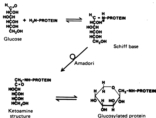
FIG. 1. Proposed reaction scheme for nonenzymatic glycosylation of albumin.
