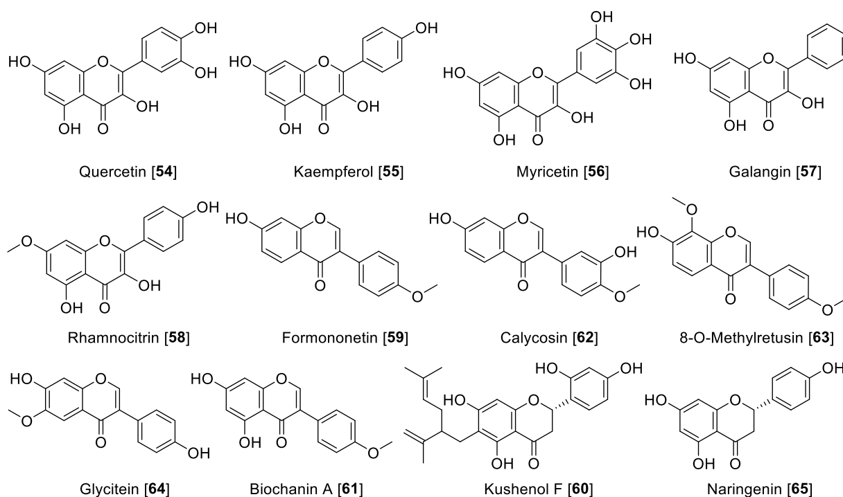
Figure 7. Chemical structure of selected flavanol, isoflavone, and flavanone MAO inhibitors.
