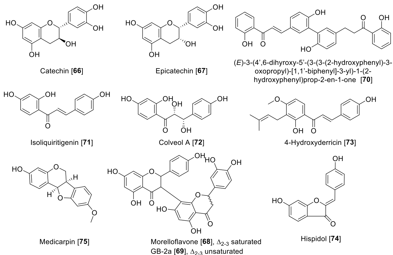
Figure 8. Chemical structure of selected miscellaneous flavonoid MAO inhibitors.
