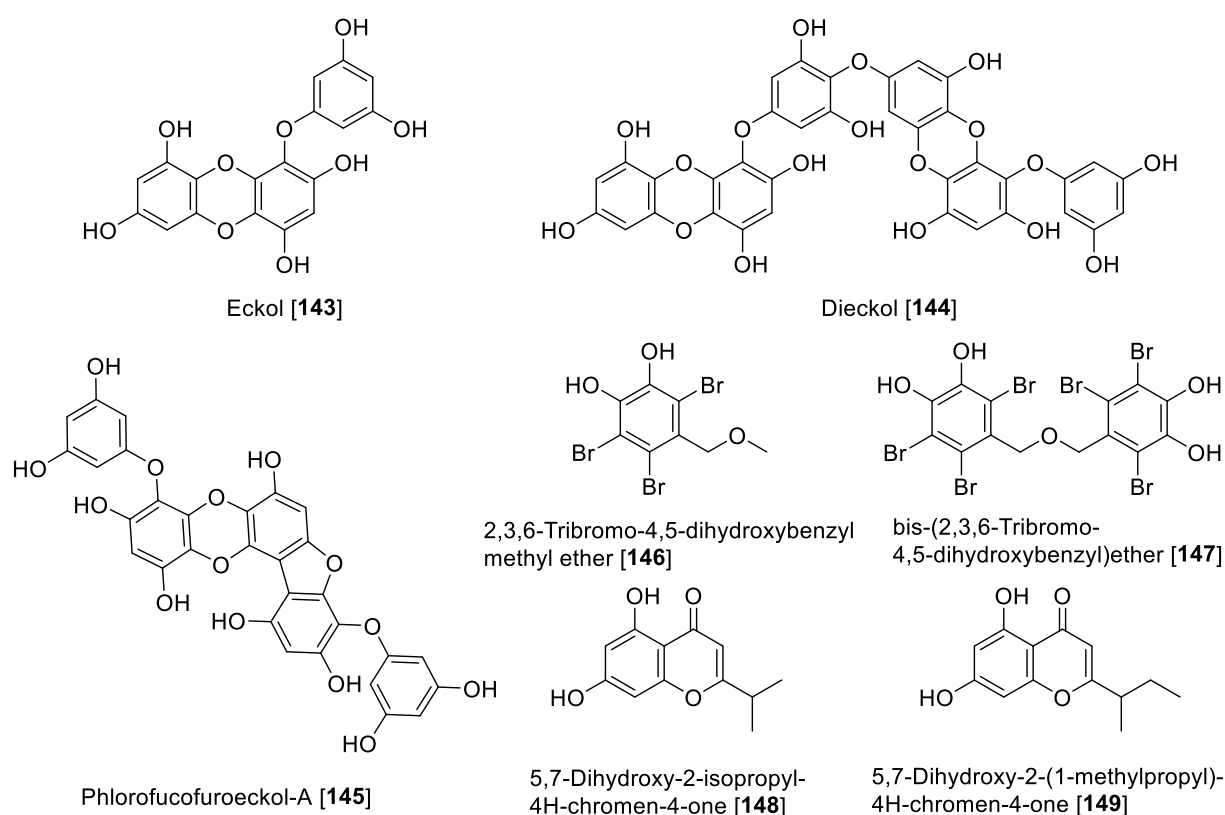
Figure 14. Chemical structure of selected marine isolated compound MAO inhibitors.
