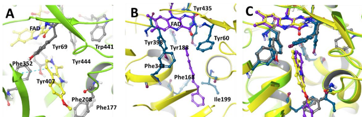
Figure 2. Active site configuration of human (A) MAO-A (PDB structure 2Z5X) with harmine and (B) MAO-B (PDB structure 1OJ9) with 1,4,-diphenyl butene, depicting key amino acids lining the enzyme active site. (C) Overlaid view of MAO-A and MAO-B substrate binding site. Harmine and 1,4,-diphenyl butene are selective reversible inhibitors of MAO-A and MAO-B, respectively.
