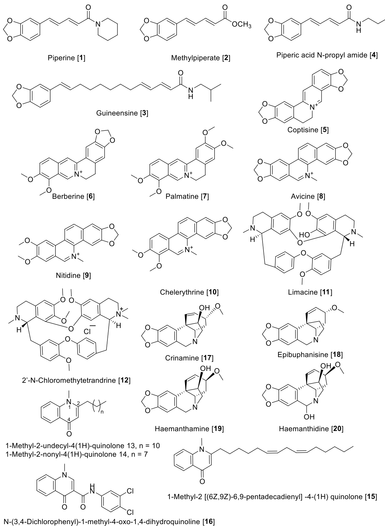
Figure 4. Chemical structure of selected alkaloid MAO inhibitors with piperine, quinolone, and isoquinoline skeletons.
