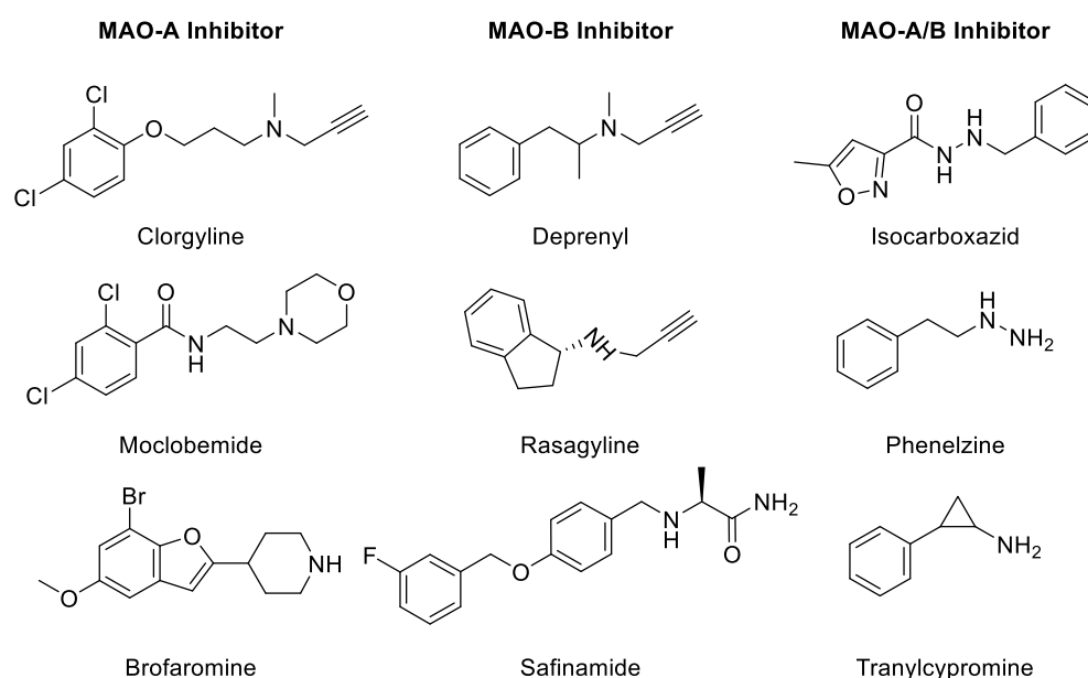
Figure 3. Chemical structure of selected MAO inhibitors.
