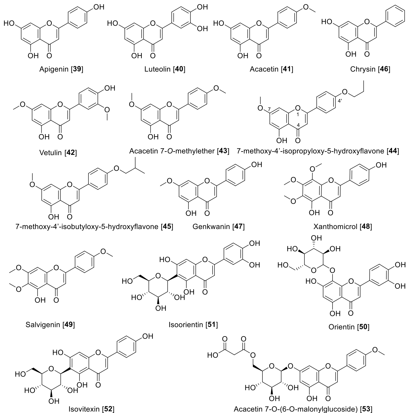
Figure 6. Chemical structure of selected flavone MAO inhibitors.
