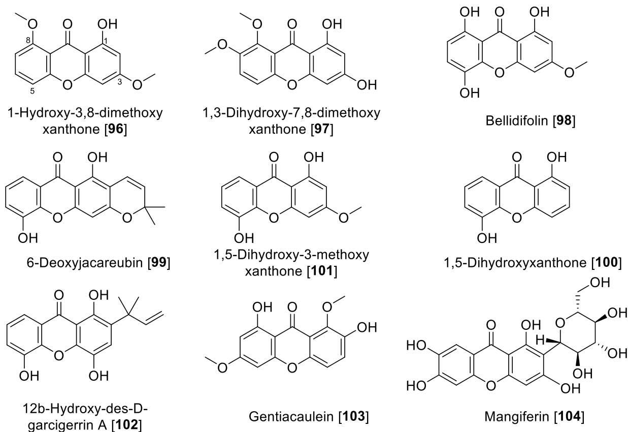
Figure 10. Chemical structure of selected xanthone MAO inhibitors.
