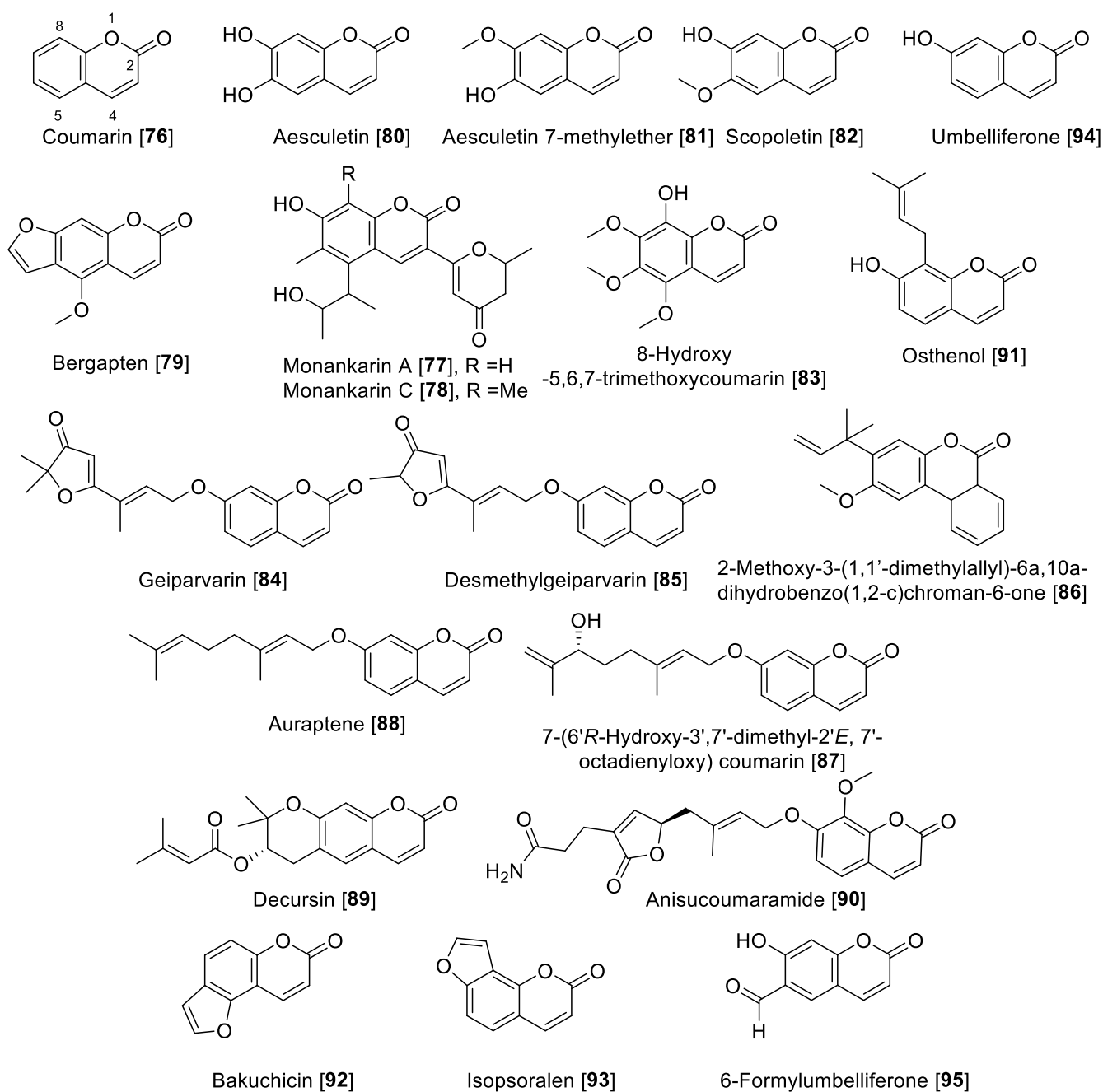
Figure 9. Chemical structure of selected coumarin MAO inhibitors.
