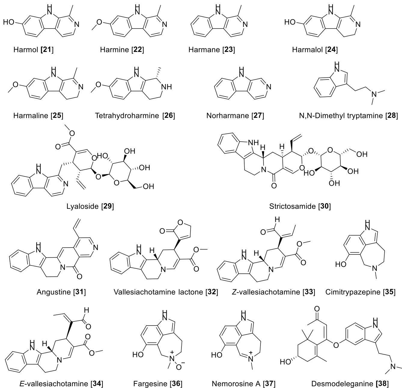
Figure 5. Chemical structure of selected alkaloid MAO inhibitors with indole motif.
