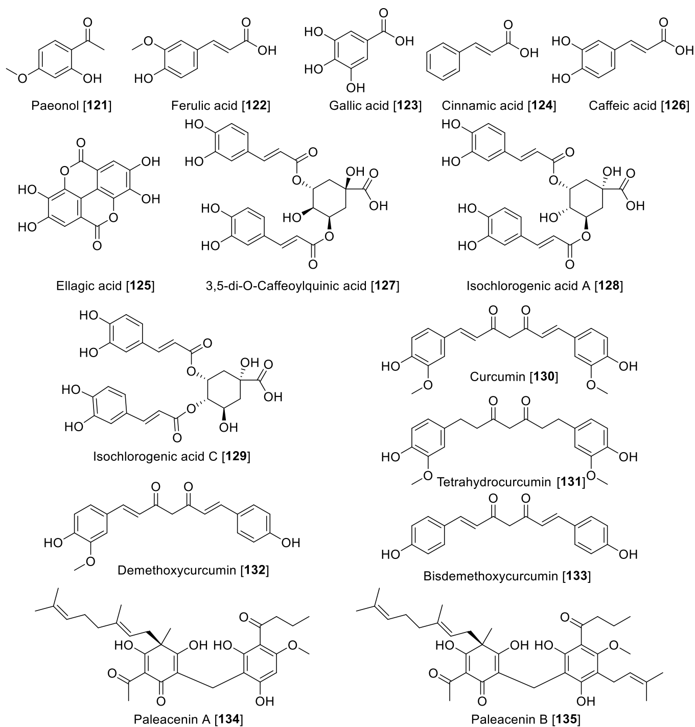
Figure 12. Chemical structure of miscellaneous polyphenol MAO inhibitors.
