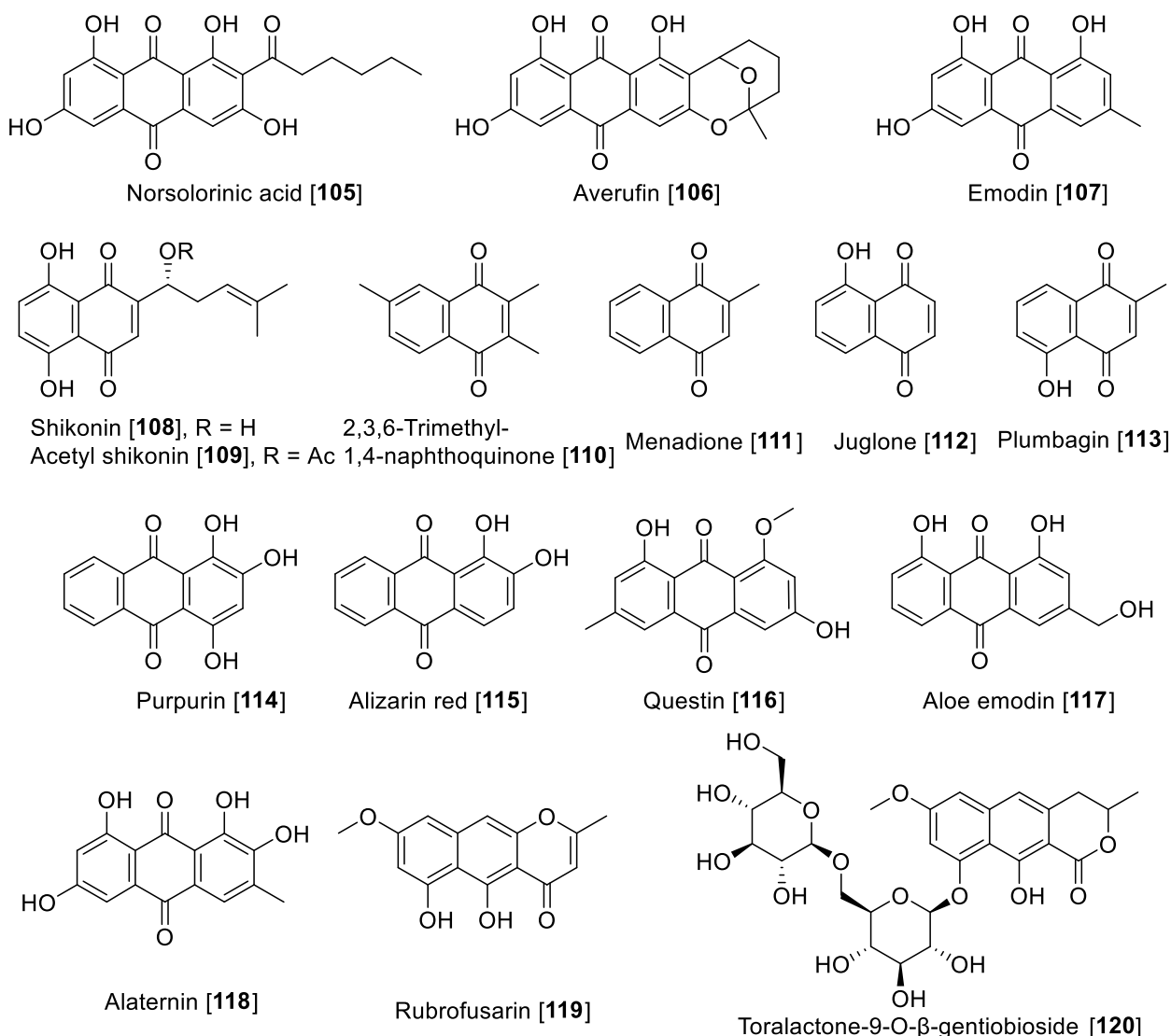
Figure 11. Chemical structure of selected naphthoquinone and anthraquinone MAO inhibitors.
