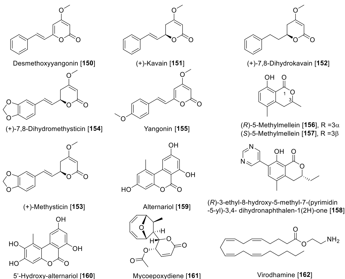
Figure 15. Chemical structure of selected miscellaneous compound MAO inhibitors.
