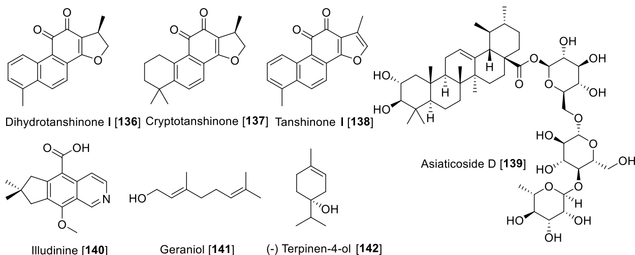
Figure 13. Chemical structure of selected terpenoid MAO inhibitors.
