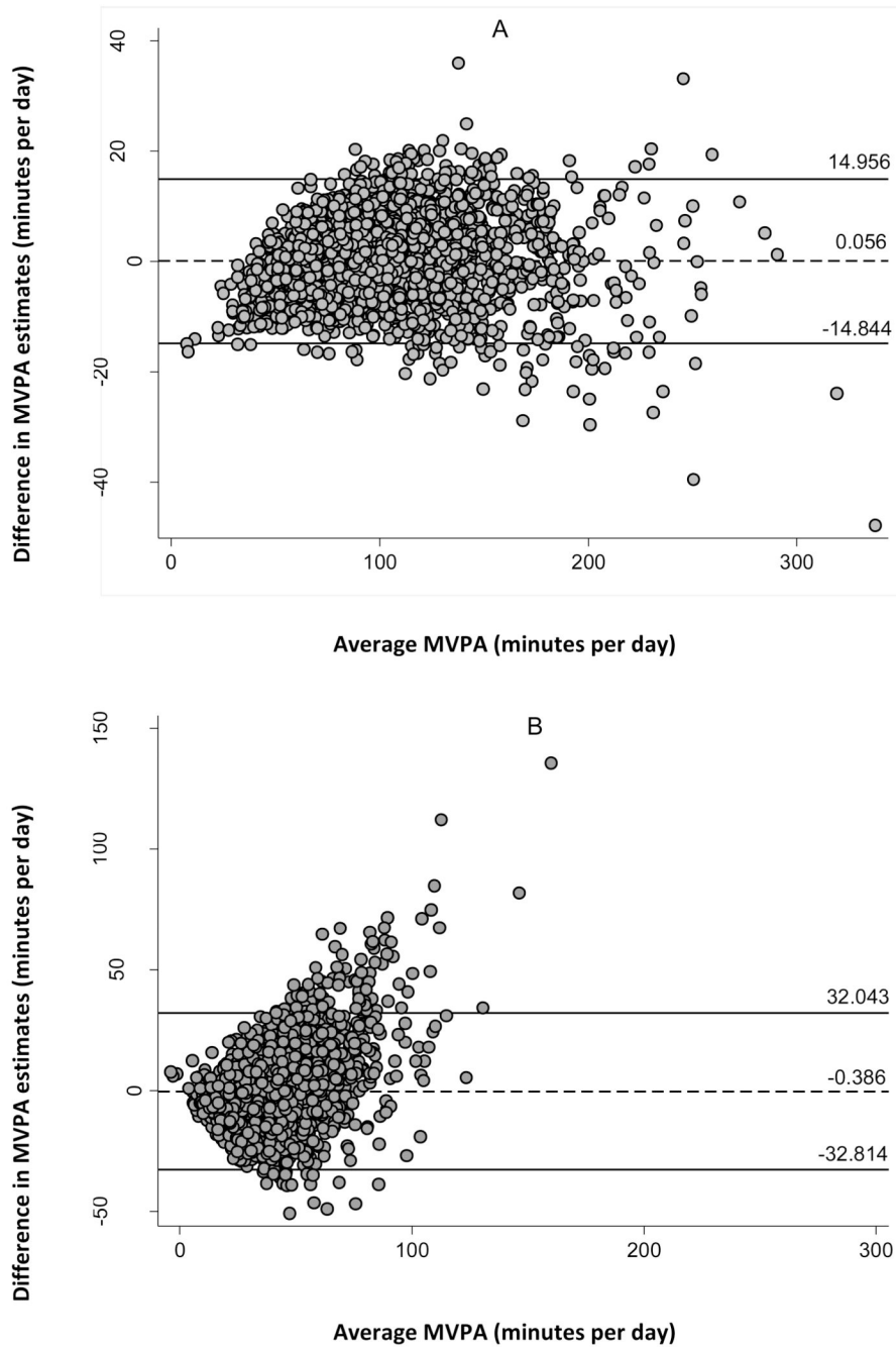
Figure 1. Bland Altman plots comparing the actual MVPA estimate vs. the predicted MVPA estimate from other cutpoints. These plots represent the best and worst models from Table 1.
