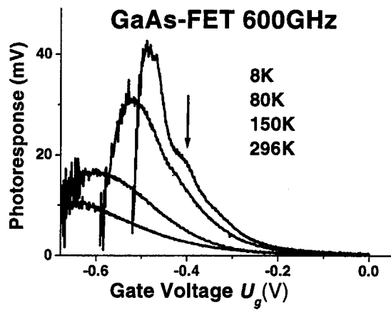
FIG. 1. Measured photoresponse of the GaAs/AlGaAs 0.15 μm FET for the 600 GHz radiation. Radiation induced source-drain voltage as a function of the gate voltage U_g is shown for temperatures of 8, 80, 150, and 296 K. The arrow marks the maximum corresponding to the resonant detection observed at the lowest temperature: 8 K.
