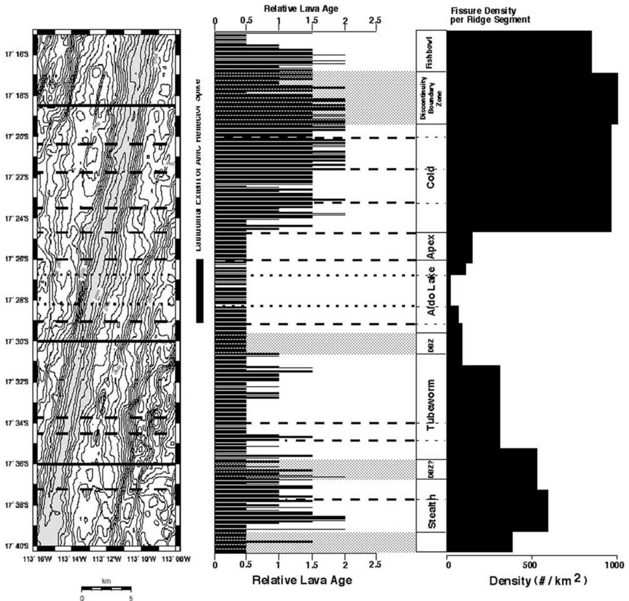
Figure 4. Distribution of tectonic and volcanic features along the southern EPR crest at 17^{\circ}15'–40'S , modified from R. M. Haymon et al. (manuscript in preparation, 2001). Bathymetric contour interval is 20 m, from the Sea Beam 2000 data of Scheirer et al. [1996b]. Shading indicates areas shallower than 2700 m. Solid horizontal lines over bathymetry indicate central latitudes of distinct third-order discontinuities [after White et al., 2000], dashed lines indicate distinct fourth-order discontinuities, and dotted lines indicate potential fourth-order discontinuities (both after White et al. [2001]). Vertical, solid bar to the right of bathymetry indicates latitudinal extent of AMC reflector spike [Mutter et al., 1995]. Moving to the right, the next column shows the along-axis variation in inferred relative lava age (after R. M. Haymon et al., manuscript in preparation, 2001). Each small histogram bar represents the minimum relative lava age within a 100-m latitudinal bin. Third-order discontinuities are shaded zones (including discontinuity boundary zones, DBZs), distinct fourth-order discontinuities are dashed lines, and potential fourth-order discontinuities are dotted lines. The last two columns show the locations of “Deval”-bounded ridge segments, as determined by White et al. [2001], and a horizontal histogram of the fissure density per ridge segment.
