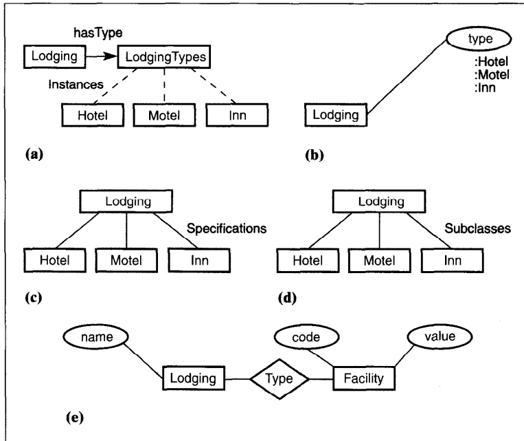
Figure 5. Possible representations in Cyc and resource schemas for the same concept, each allowing a different aspect of it to be emphasized: (a) Cyc concept represented as a slot; (b) Schema concept represented as an attribute; (c) Cyc concept represented as a category; (d) Schema concept represented as a class; and (e) Schema concept represented as a relationship.
