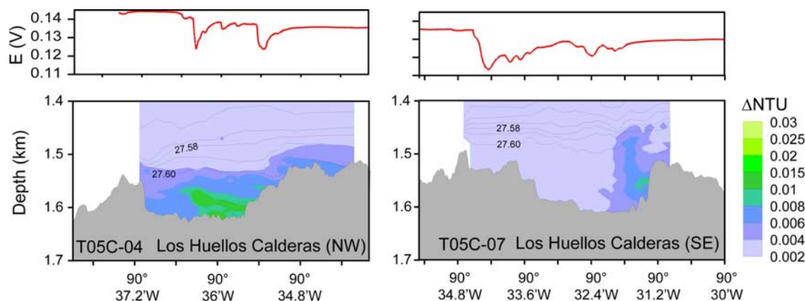
Figure 6. Hydrothermal plumes over the Los Huellos calderas on the east limb of the GSC. (top) Profiles of E from DSL-3. (bottom) Contoured \Delta NTU data from CTDOs through the calderas. The CTDO towpaths closely followed the DSL towpath. Potential density isopycnals are overlain.
