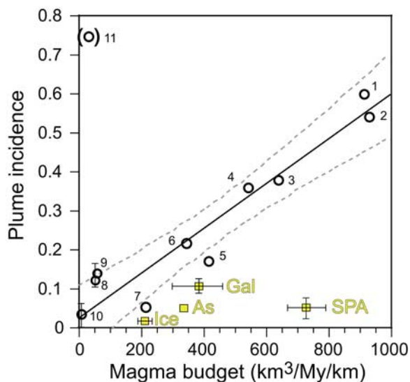
Figure 8. Scatterplot of p_h versus magma budget, V_m (spreading rate \times crustal thickness), for “normal” ridge sections (black circles) and hot spot-affected ridge sections (yellow squares). Hot spot sections include “Ice,” Reykjanes Ridge ( 58^\circ – 63^\circ N); “As,” MAR 7^\circ – 11^\circ S; “Gal,” GSC (this study); and “SPA,” SEIR ( 37^\circ – 39.5^\circ S). Normal ridge sections include 1, EPR 13^\circ – 18^\circ S; 2, EPR 27^\circ – 32^\circ S; 3, EPR 9^\circ – 13^\circ N; 4, EPR 15^\circ – 18^\circ N; 5, SEIR, 77^\circ – 88^\circ E; 6, JdFR; 7, MAR 2 – 7^\circ S [German et al. , 2005]; 8, western SWIR ( 58^\circ – 66^\circ E); 9 and 10, oblique ( 10^\circ – 16^\circ E) and orthogonal ( 16^\circ – 23^\circ E) supersegments, respectively, of eastern SWIR; and 11, Gakkel Ridge. References for these sections are provided by Baker et al. [2004], except for 7. Solid line is least squares regression for normal ridges, p_h = 0.04 + 0.00055V_m ; dotted lines are the 95% confidence bands for the slope. The Gakkel Ridge value ( p_h = 0.75 ) is not used because it is inflated by unique hydrographic and bathymetric characteristics [Baker et al. , 2004].
