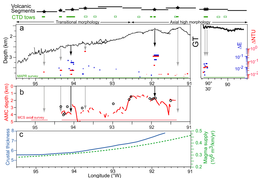
Figure 3. (a) Bathymetric cross-section of the GSC in our study area. The Galápagos hot spot influence is centered near the Galápagos Transform (GT), where it creates a shallow ridge and axial high morphology. Location and intensity of \Delta NTU (red lines) and \Delta E (blue lines) plume anomalies are plotted beneath the bathymetry; logarithmic scales for each are at far right. Thin lines indicate that the \Delta NTU anomaly was seen only on the lowermost MAPR ( \sim 50 mab); all other \Delta NTU anomalies were detected on multiple MAPRs. Black vertical arrows show vent sites confirmed by camera tows (Haymon et al., submitted manuscript, 2008); gray arrows show sites where plume data strongly suggest active venting. At the panel top are shown the location of CTD tows, solid where plumes were detected and hollow where not detected, and the volcanic segmentation (White et al., submitted manuscript, 2008), with stars marking confirmed and possible vent sites. (b) Red profile traces the depth of the AMC from along-axis seismic lines, and hexagons mark the depth from cross-axis seismic lines [Detrick et al., 2002; Blacic et al., 2004]. (c) Magma supply (green dotted line) and crustal thickness (blue solid line) both increase toward the maximum hot spot influence [Canales et al., 2002; Sinton et al., 2003].
