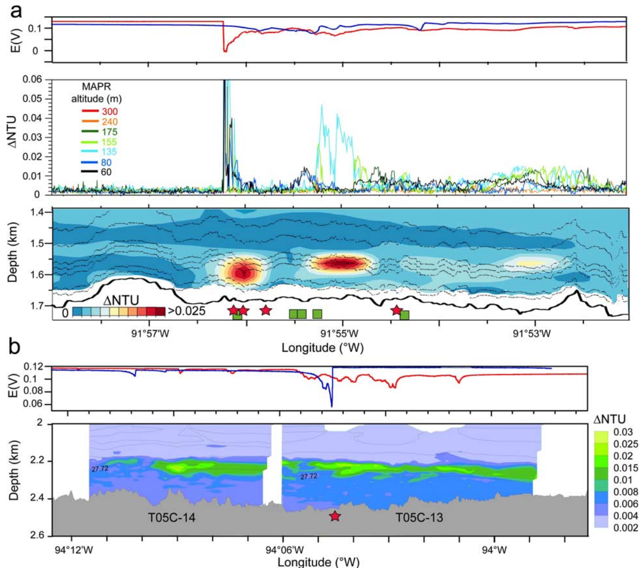
Figure 5. (a) Hydrothermal plumes over the Iguanas/Pinguinos vent field. Top panel shows profiles of E from DSL-2 (red line) and DSL-6 (blue line). As apparent during DSL-2, moving west to east, the ORP detector reacts quickly upon encountering reduced chemicals but has a slow recovery to background values. Middle panel shows individual MAPR records, color coded to depth above bottom. Bottom panel shows the same data contoured; parallel lines above the seafloor indicate the MAPR paths. Red stars are active vents, and green boxes are vent faunal communities imaged by a camera survey ( 91^{\circ}53.5' - 56.5'W ) (Haymon et al., submitted manuscript, 2008). (b) Hydrothermal plumes over the Navidad vent field ( 94^{\circ}04.5'W ) (Haymon et al., submitted manuscript, 2008). Top panel shows profiles of E from DSL-2 (red line) and DSL-6 (blue line). Bottom panel shows contoured \Delta NTU data from CTDO tow-yos showing a strong plume layer extending for >20 km at a depth of \sim 2200 - 2300 m. Potential density isopycnals are overlain. Red star is the active vent. Note change in \Delta NTU color scale compared to Figure 5a.
