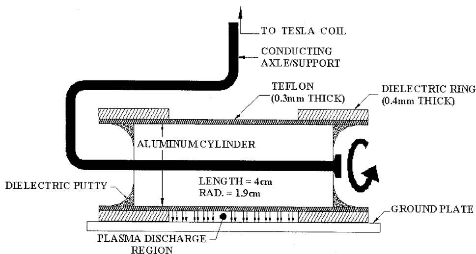
FIG. 1. Schematic of cold plasma device.
