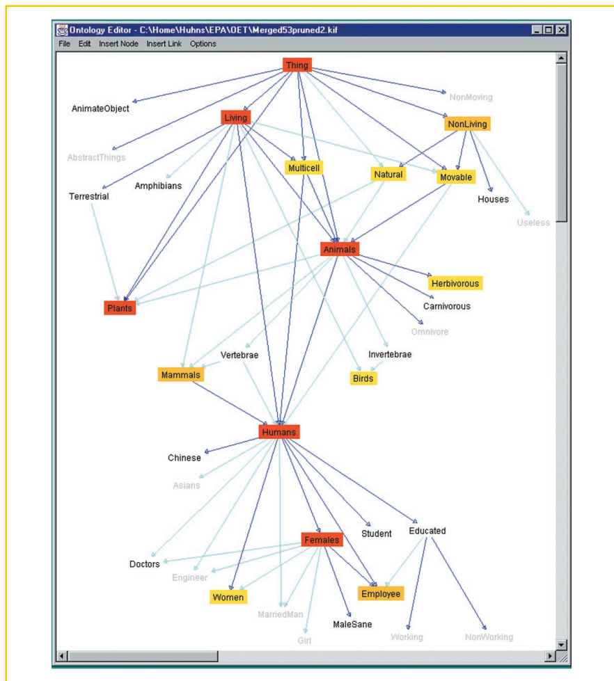
Figure 4. Consensus ontology. Weakly reinforced concepts were removed and concepts with common subclasses and superclasses were merged to produce this graph containing 36 classes related by 62 subclass links.
