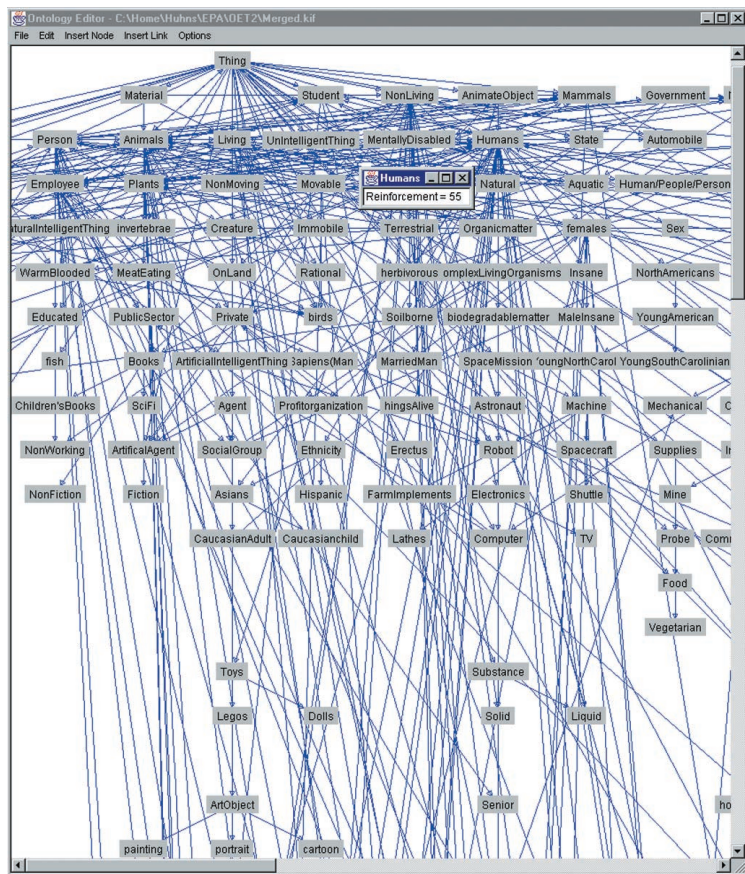
Figure 3. Merged ontology from 55 independently constructed ontologies for the People domain. Of 281 classes, 38 with 71 subclass links appear more than once.
