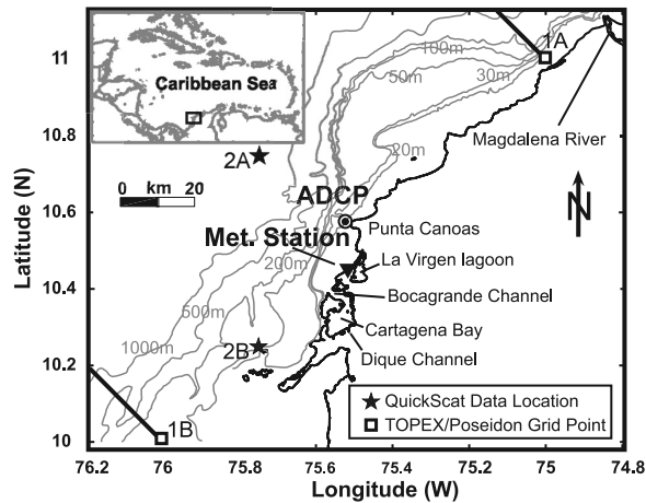
Figure 1. Study area showing instrument deployment sites, locations of buoyancy fluxes, points of QuickScat and TOPEX/Poseidon data utilized and transect locations used to carry out momentum balance analyses (for details see text).
