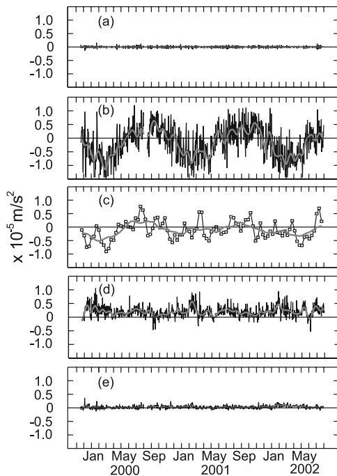
Figure 4. Comparison of cross-shelf momentum terms. (a) Acceleration ( \partial v/\partial t ); (b) Coriolis ( fu ); (c) pressure gradient ( -1/\rho_o \partial P/\partial y ); (d) wind stress ( \tau^{sy}/\rho_o h ) and (e) bottom stress ( -\tau^{by}/\rho_o h ) term. Gray bold lines represent low pass filtered time series with a cut-off period of 1 month.
