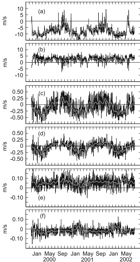
Figure 3. (a) Along-shelf and (b) cross-shelf components of surface wind velocities from QuikScat data in location 2B (see Figure 1). Along-shelf component of (c) near surface and (d) near the bottom current velocities. Cross-shelf component of (e) near surface and (f) near bottom current velocities. Gray bold lines represent low pass filtered time series with a cut-off period of 1 month.
