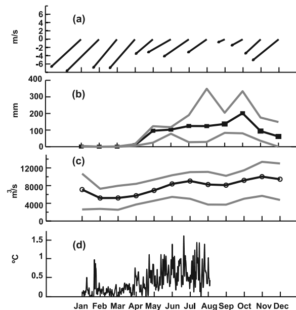
Figure 2. Multi-annual (1999–2002) monthly-averaged data. (a) Vectors of surface winds from QuikScat (grid point 2B); (b) maximum, mean and minimum accumulated precipitation; and (c) maximum, mean and minimum discharge of Magdalena river (1996–2000). (d) Difference in sea temperature between surface and bottom thermistors.
