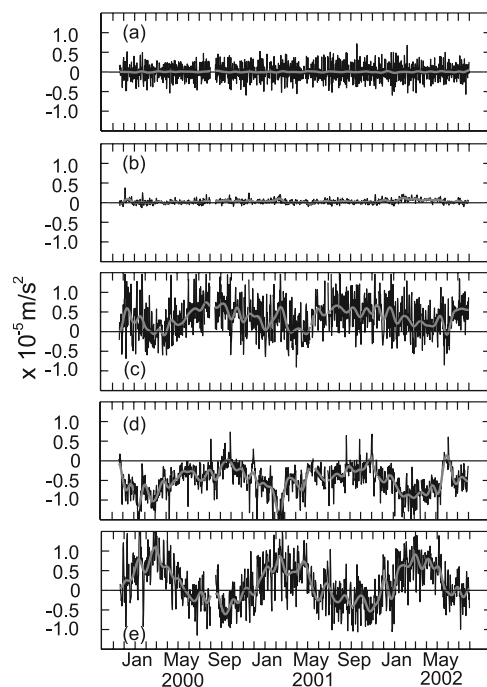
Figure 5. Comparison of along-shelf momentum terms. (a) Acceleration ( \partial u/\partial t ); (b) Coriolis ( fv ); (c) estimated pressure gradient ( -1/\rho_o \partial P/\partial x ); (d) wind stress ( \tau^{sx}/\rho_o h ); and (e) bottom stress ( -\tau^{bx}/\rho_o h ). Gray bold lines represent low-pass filtered time series with a cut-off period of 1 month.
