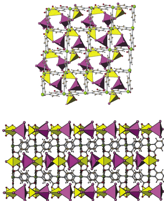
Fig. 3 View of the three-dimensional network, showing one square grid layer connected to two adjacent chains (top, view perpendicular to the layers) and the stacking of alternating layers of square grids and serpentine chains (bottom, view parallel to the layers).
