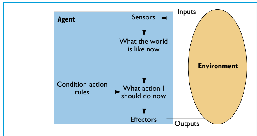
Figure 1. Simple agent-environment interaction.
