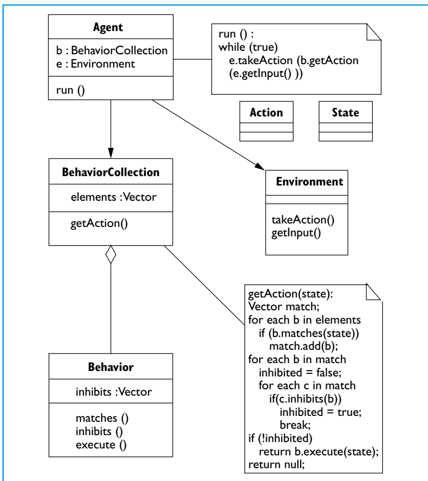
Figure 3. Diagram of a simple reactive agent.
