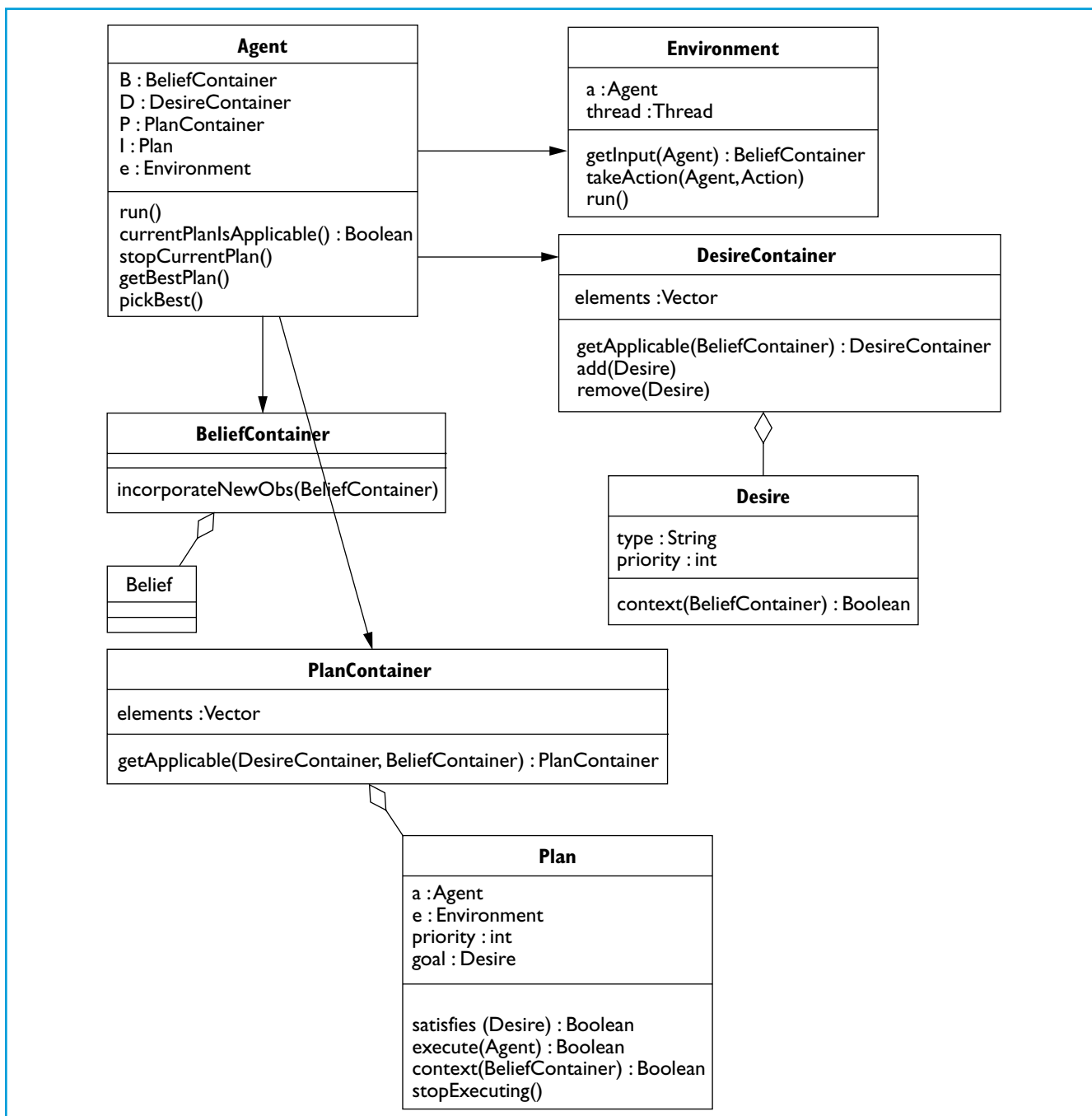
Figure 4. Diagram of a belief-desire-intention architecture.
