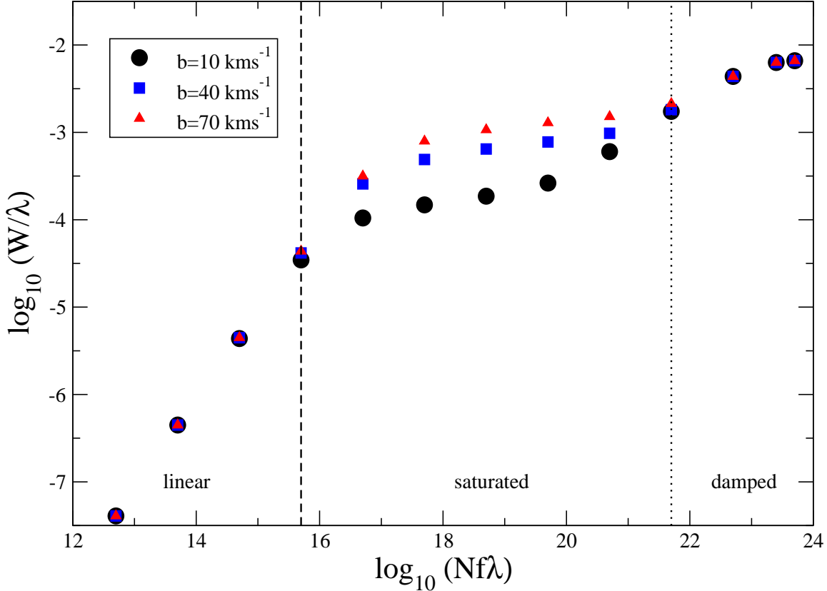
Figure 1.6 The growth function of the equivalent width with respect to the column density for the Lyman- \alpha line of Hydrogen corresponding to b-parameters of 10, 40 and 70 \text{km s}^{-1} . It can be noted that the equivalent width is independent of the b-parameter in the linear and the damped regions. The threshold between the logarithmic and the damped regions corresponds to N_{HI} \sim 10^{19} .
