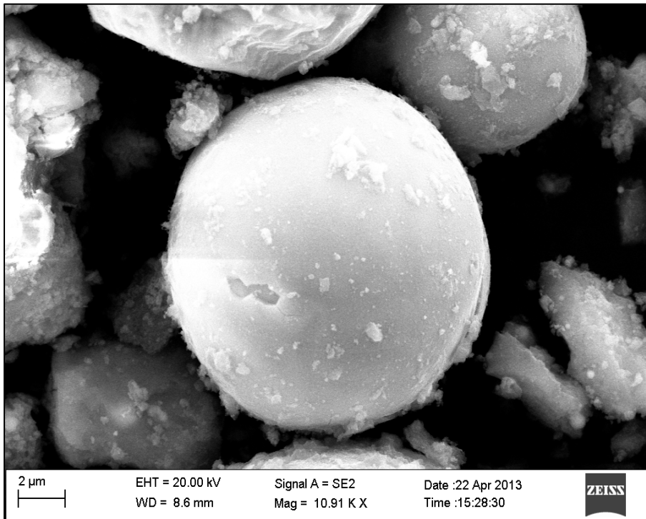
Figure 5.8: Microsphere fabricated at 25 A, with 512 \mu s pulse duration, and 64 \mu s pulse off-time. Scale indicated is 2 \mu m.
