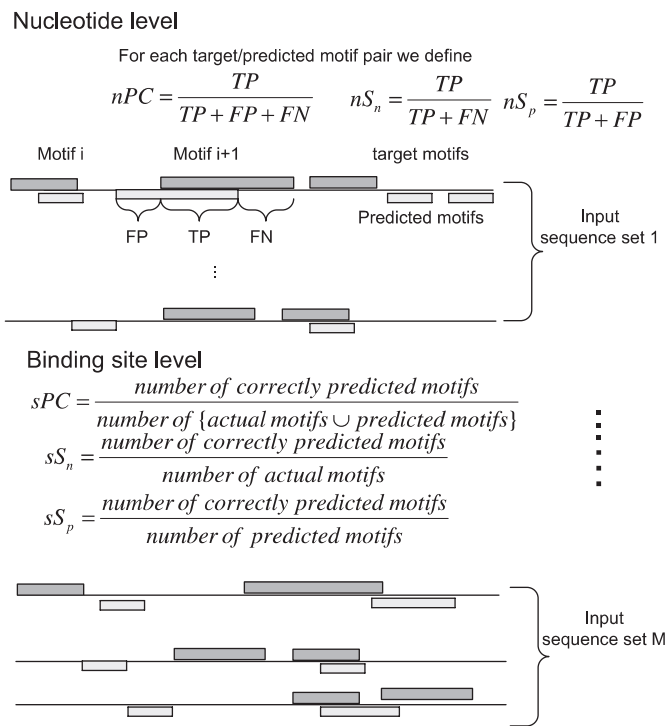
Figure 4. Measures of prediction accuracy at the nucleotide and motif levels. Accuracy scores over an input sequence set are the average accuracy scores over all its sequences. The overall accuracy scores of a motif discovery algorithm are the average accuracy scores over all M input sequence sets.
