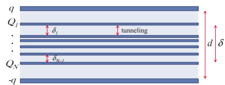
FIG. 1. (Color online) General scheme of a solid-state memcapacitor. A metamaterial medium consisting of N metal layers embedded into an insulator is inserted between the plates of a “regular” capacitor. It is assumed that the electron transfer between external plates of the capacitor (with charge \pm q ) and internal metal layers (with charges Q_k ) is negligible. Therefore, the internal charges Q_k can only be redistributed between the internal layers creating a medium polarization.
